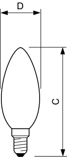
Candle B35 230V 2-25W 250lm 2700K E14ND
